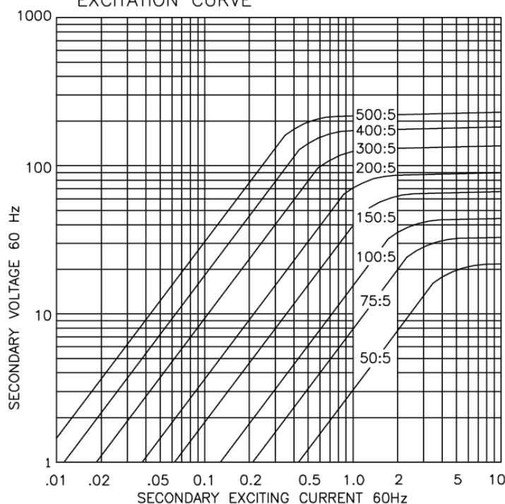
EXCITATION CURVE
