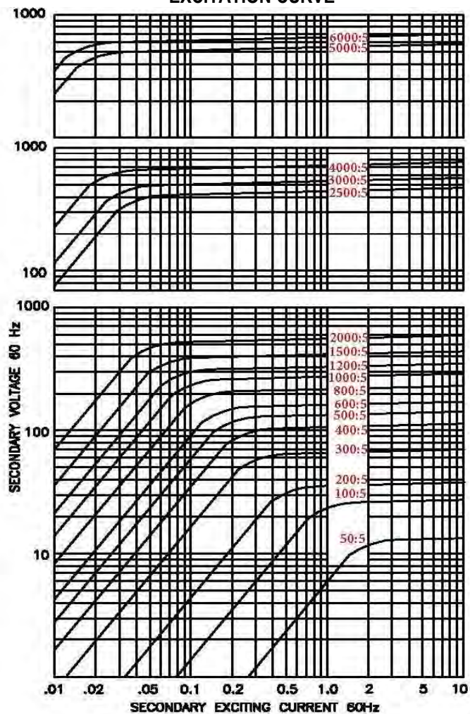
EXCITATION CURVE
