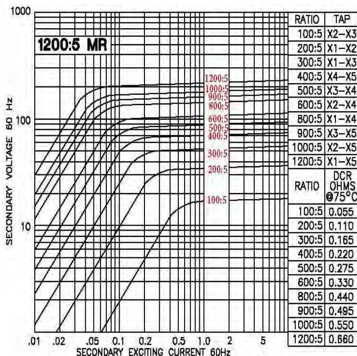
Model 115-122MR - rating C100
